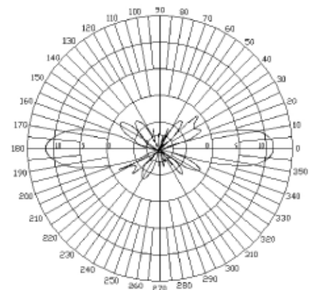
E-Plane Field Pattern
